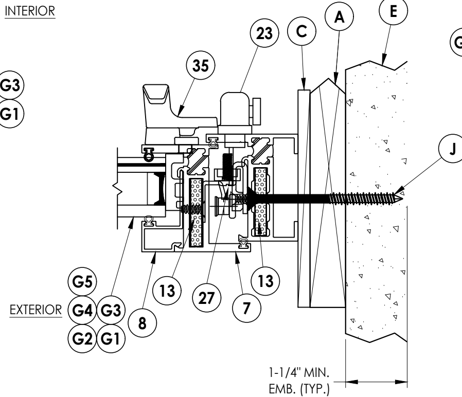
2 4 HORIZONTAL CROSS SECTION Shown w/ 1X Sub buck option
