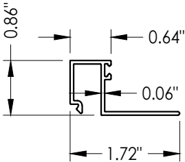
8 GLASS STOP 1-1/4"
