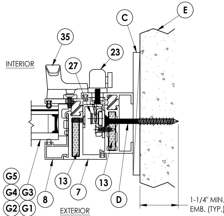
4 4 HORIZONTAL CROSS SECTION Shown w/ Direct to Masonry option
