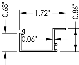
10 GLASS STOP 5/16", 7/16"
