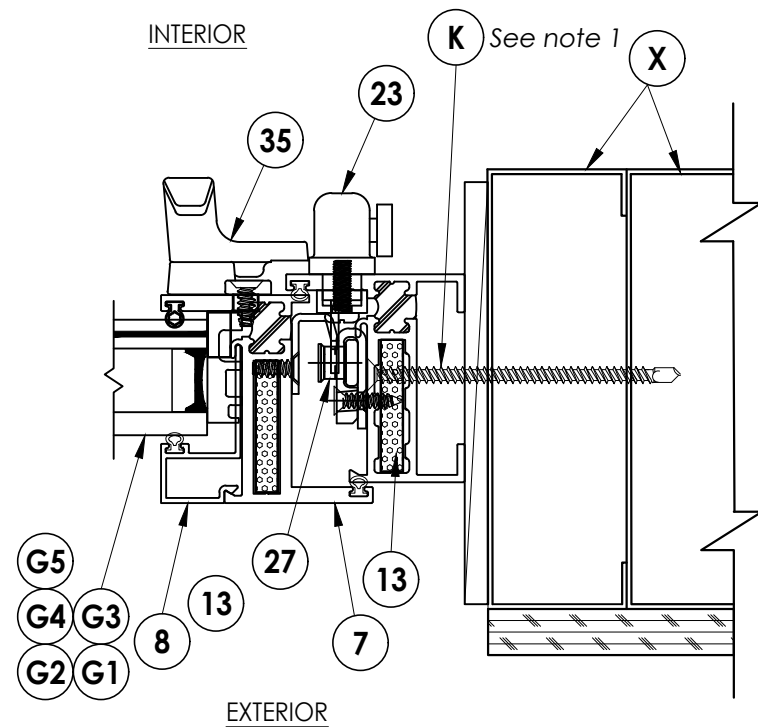
3 4 HORIZONTAL CROSS SECTION Shown w/ Steel Stud option
