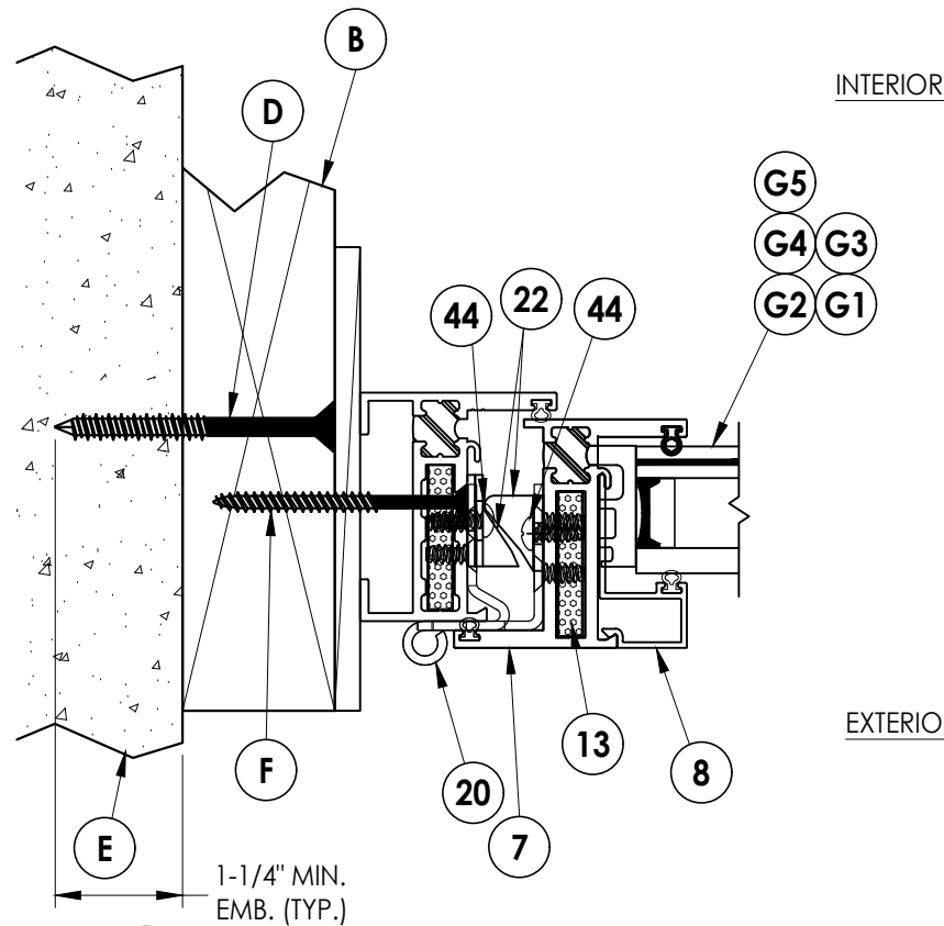
1 4 HORIZONTAL CROSS SECTION Shown w/ 2X Buck Construction
